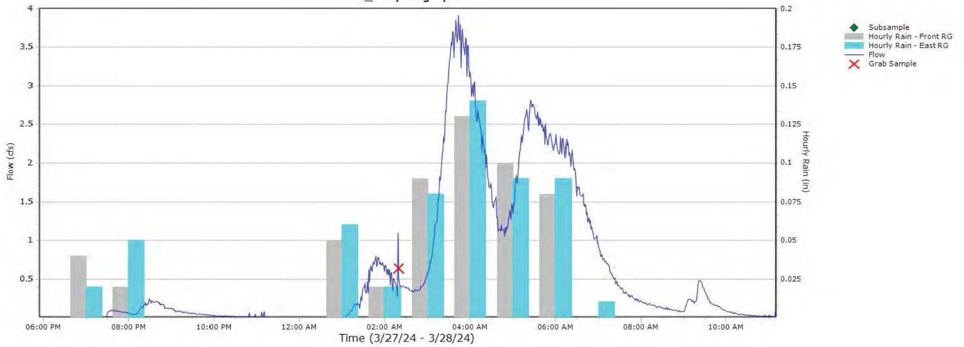
AS_6 Hydrograph
